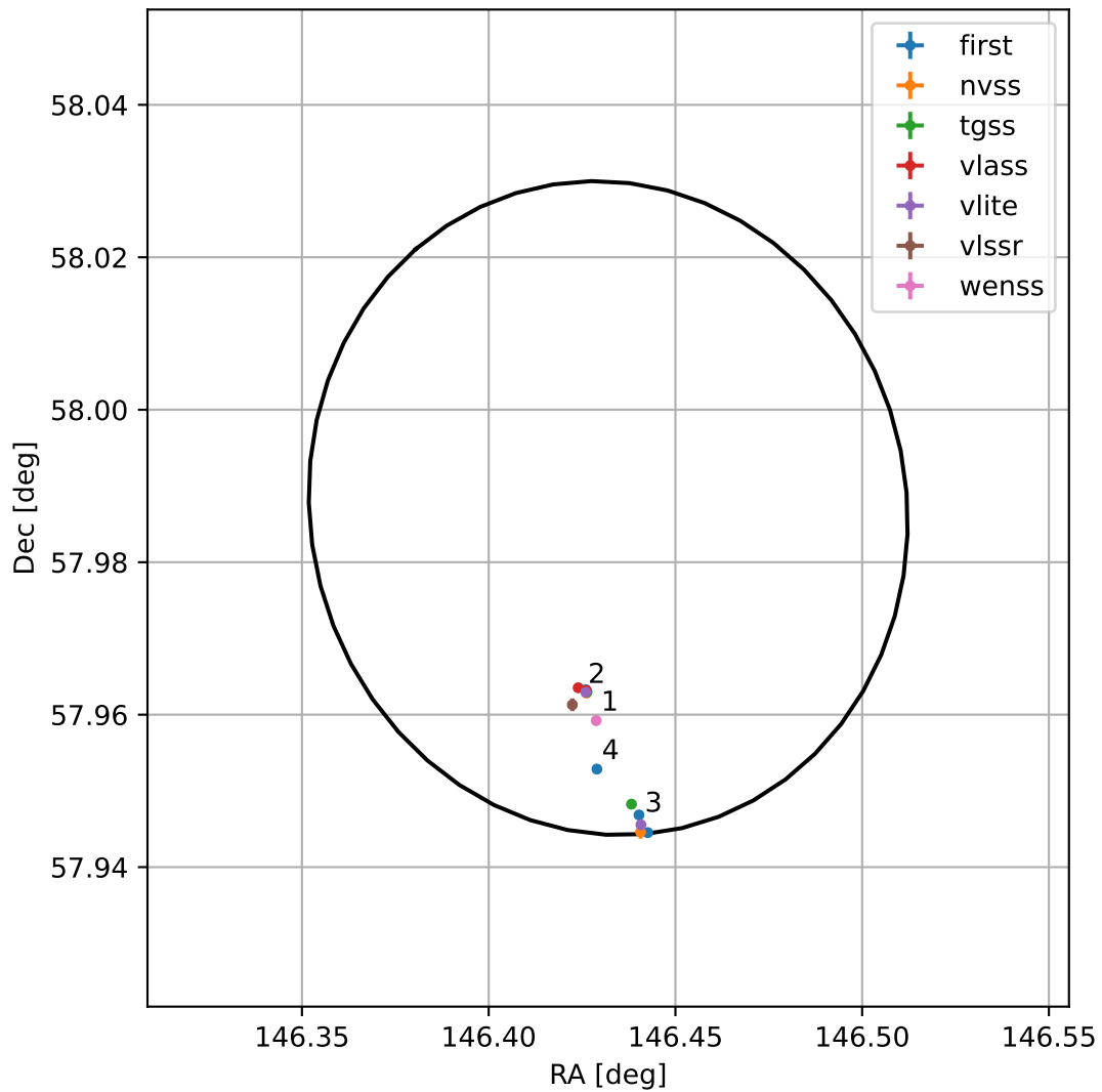
4FGL J0945.7+5759
