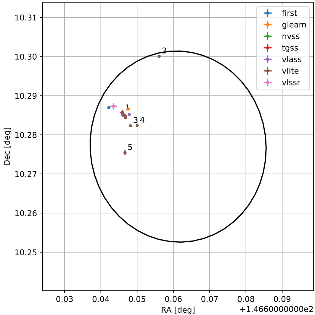
4FGL J0946.6+1016
