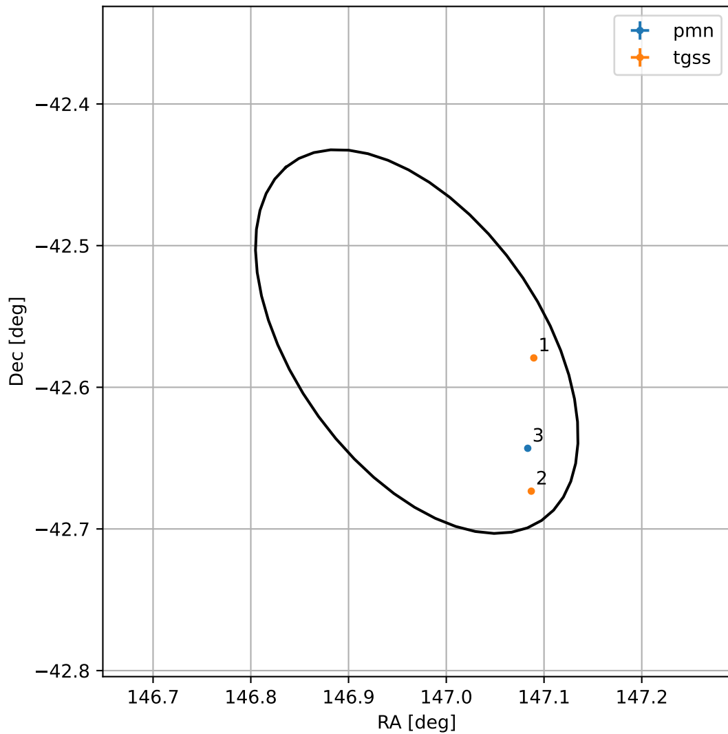
4FGL J0947.8-4234
