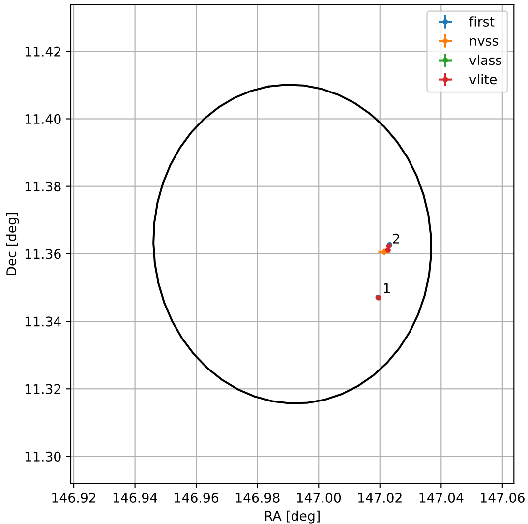
4FGL J0947.9+1121
