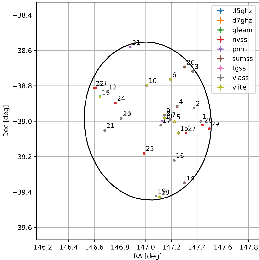
4FGL J0948.0-3859
