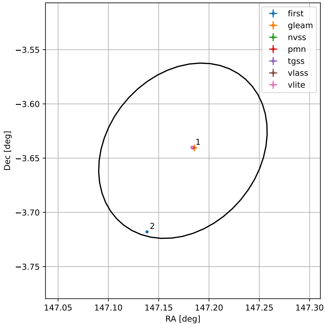
4FGL J0948.6-0338
