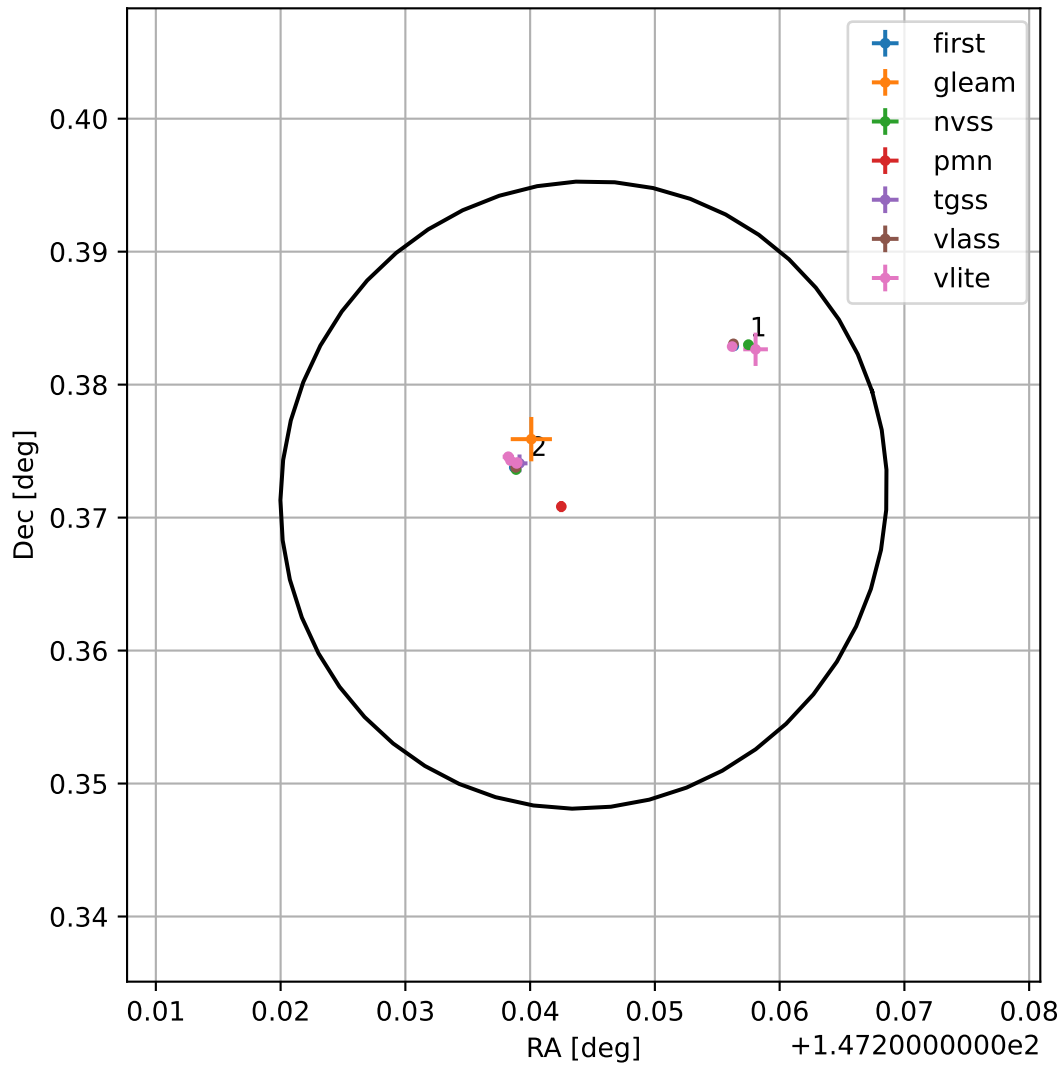
4FGL J0948.9+0022
