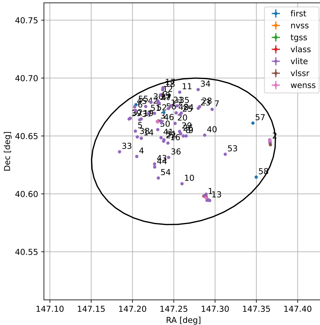
4FGL J0949.0+4038
