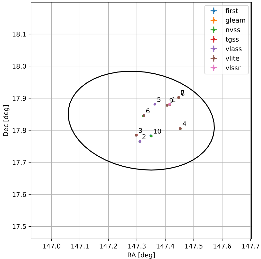
4FGL J0949.2+1749
