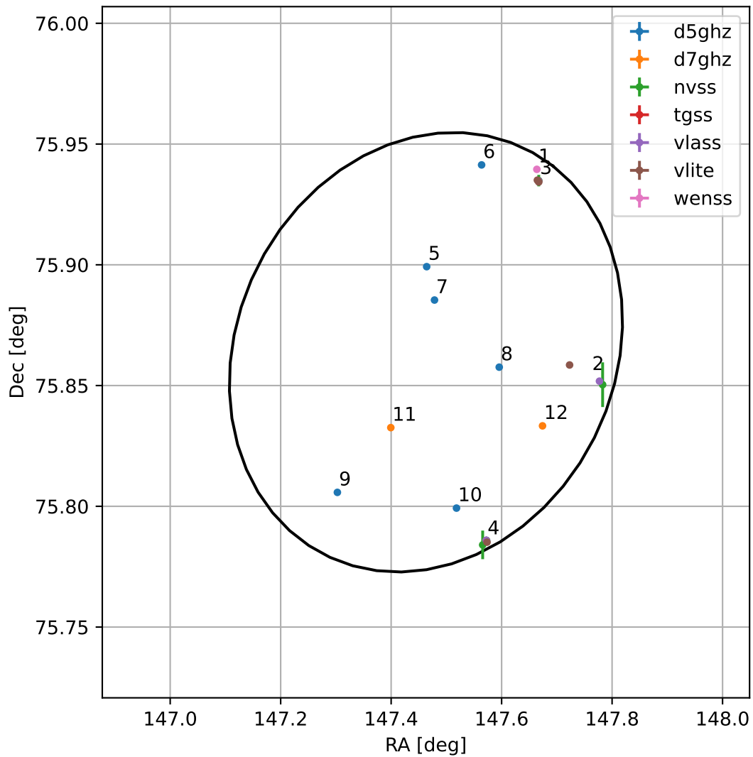
4FGL J0949.8+7551
