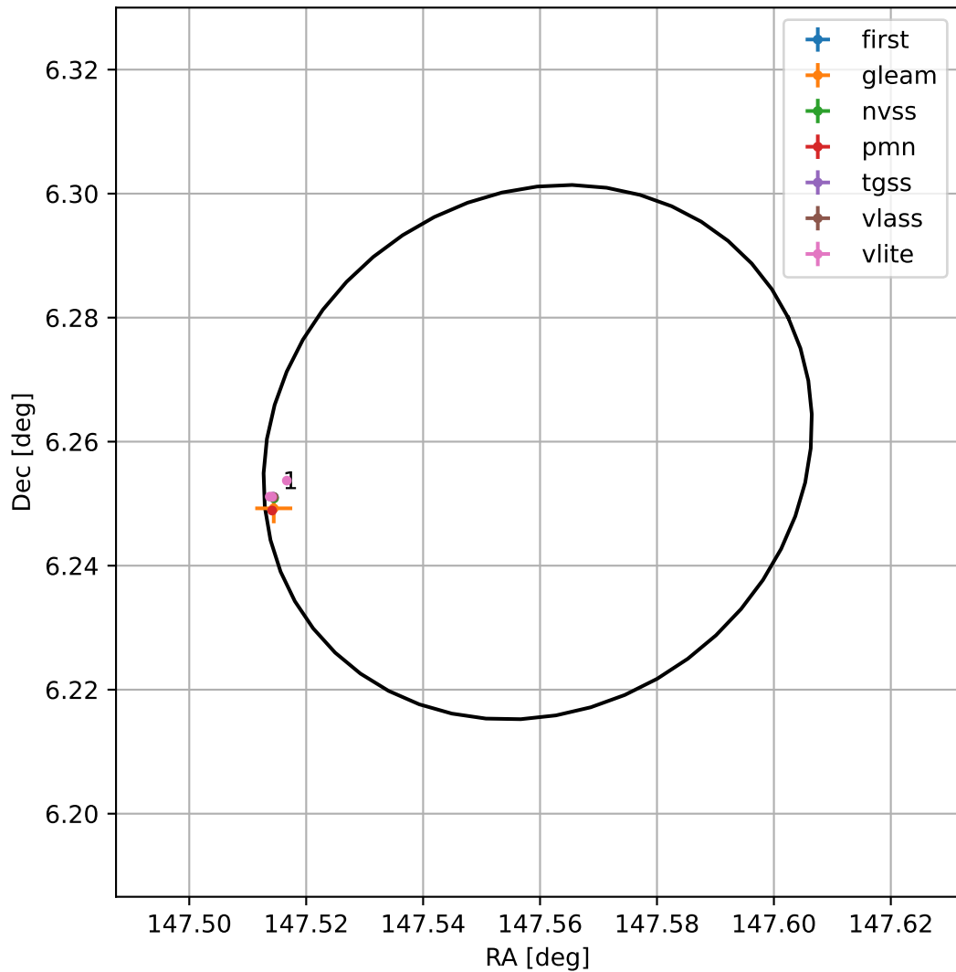
4FGL J0950.2+0615
