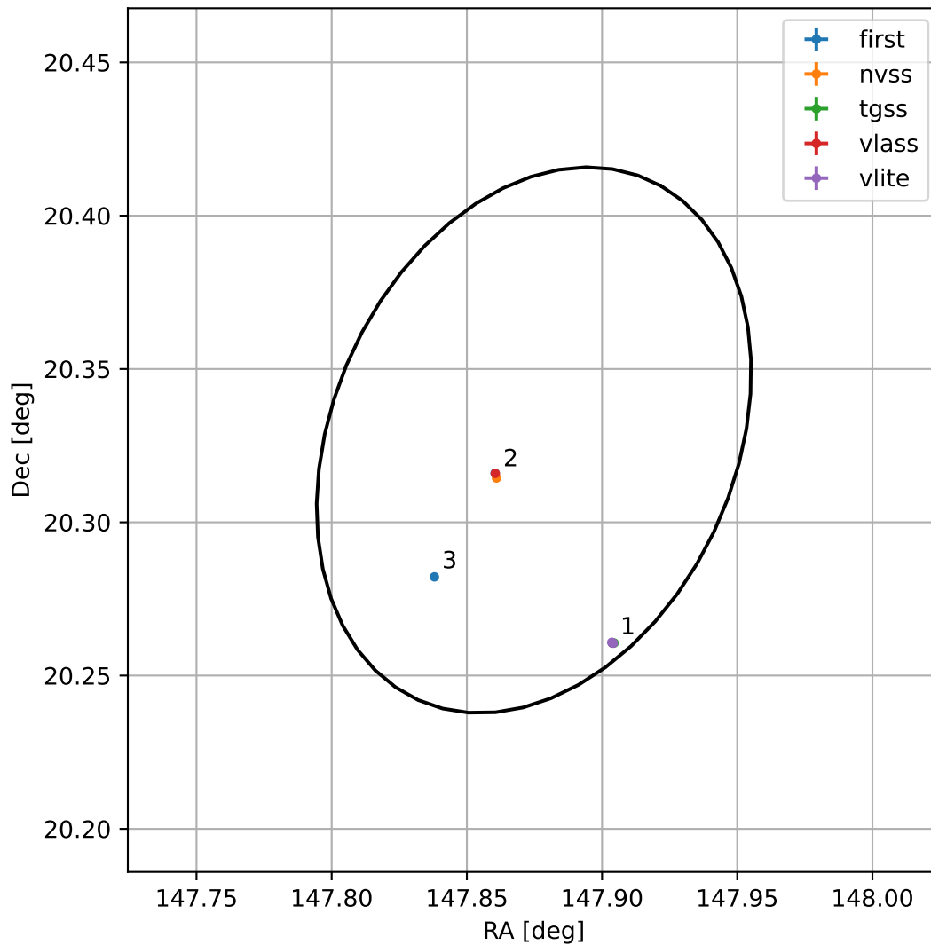
4FGL J0951.4+2019
