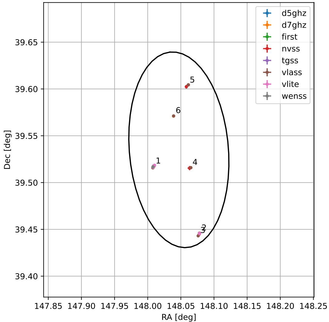
4FGL J0952.1+3932
