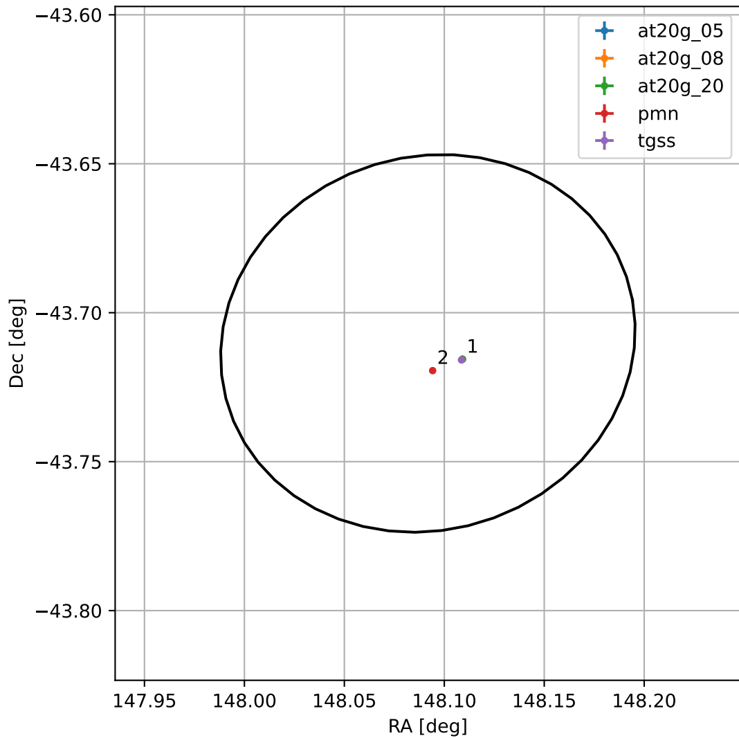
4FGL J0952.3-4342
