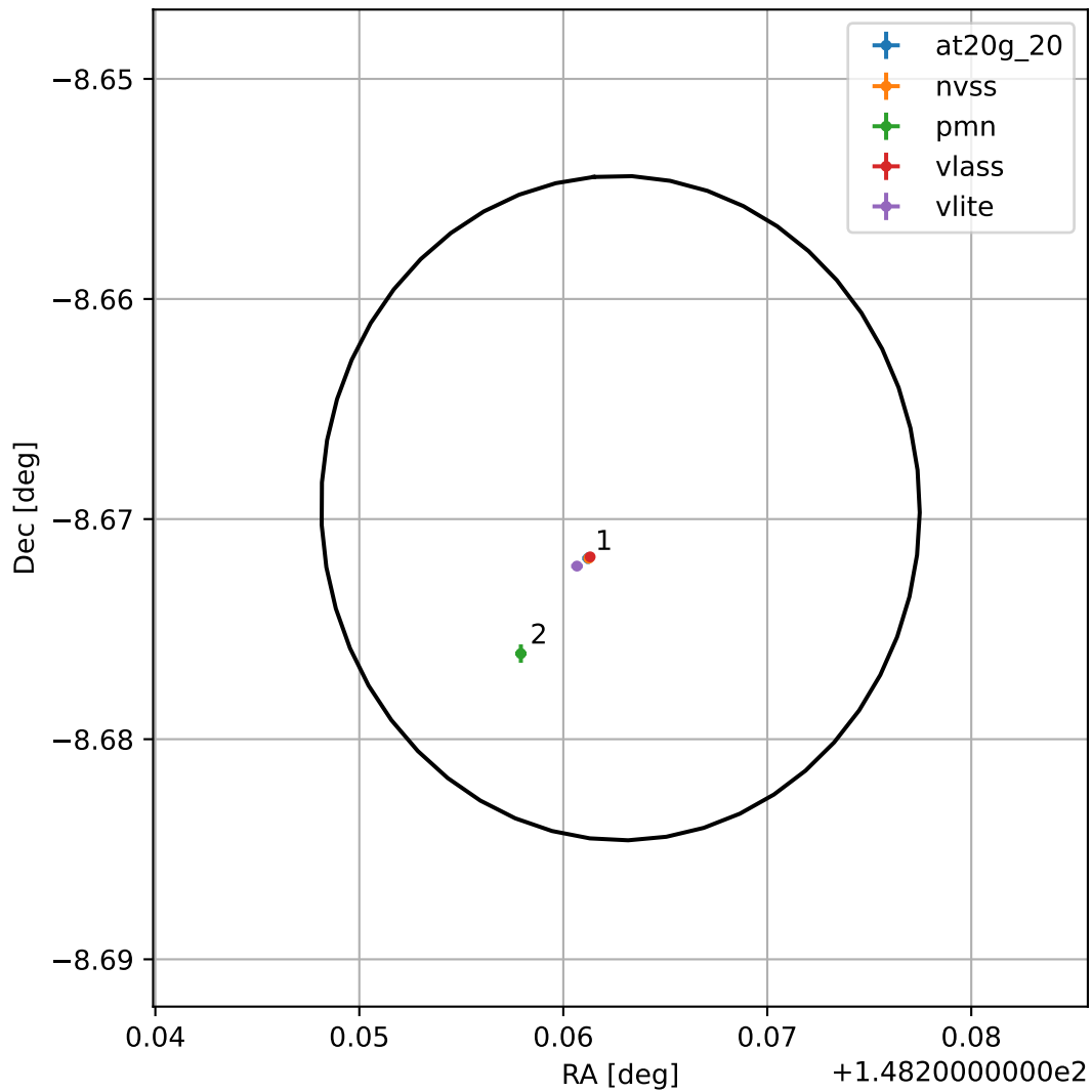
4FGL J0953.0-0840
