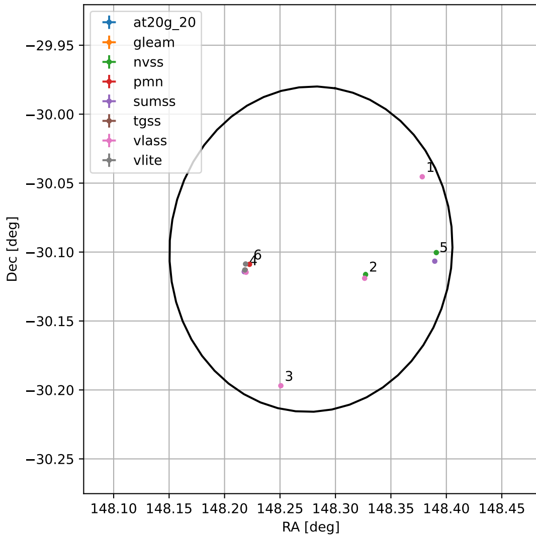
4FGL J0953.1-3005
