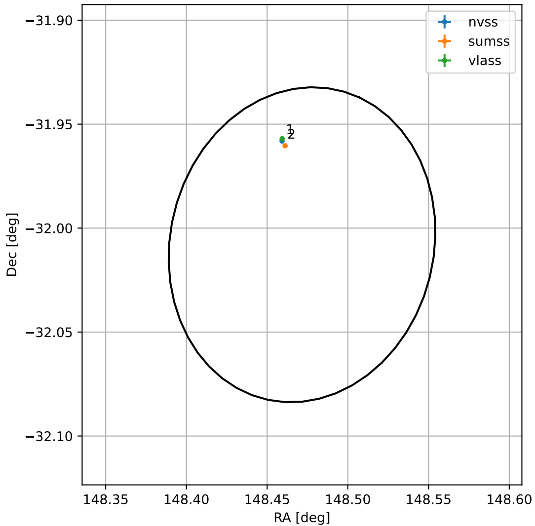
4FGL J0953.8-3200
