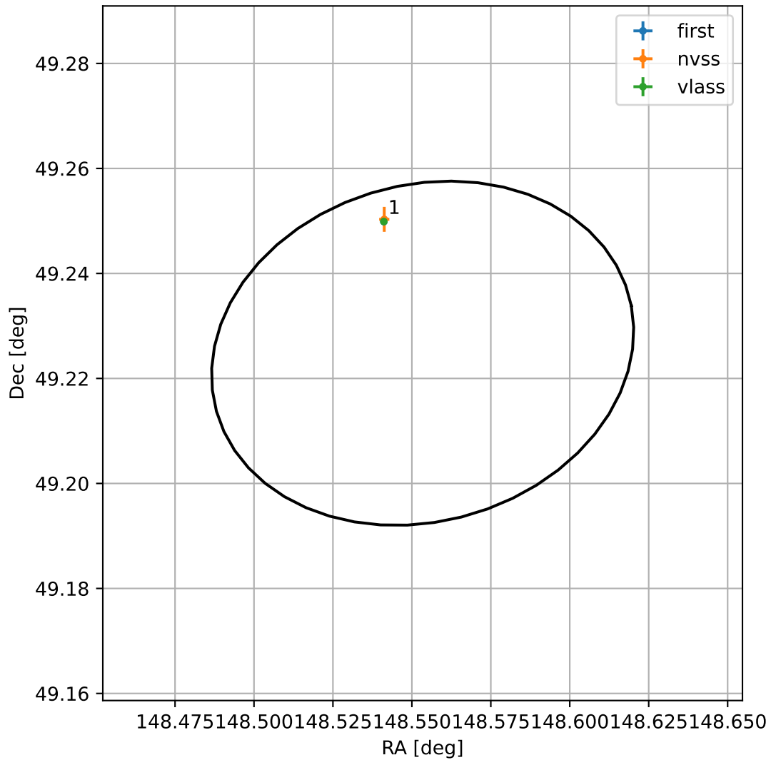
4FGL J0954.2+4913
