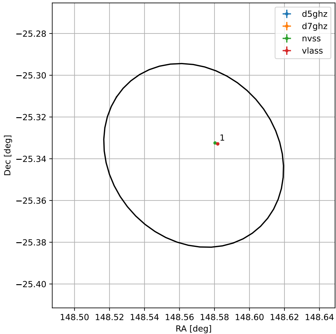
4FGL J0954.2-2520
