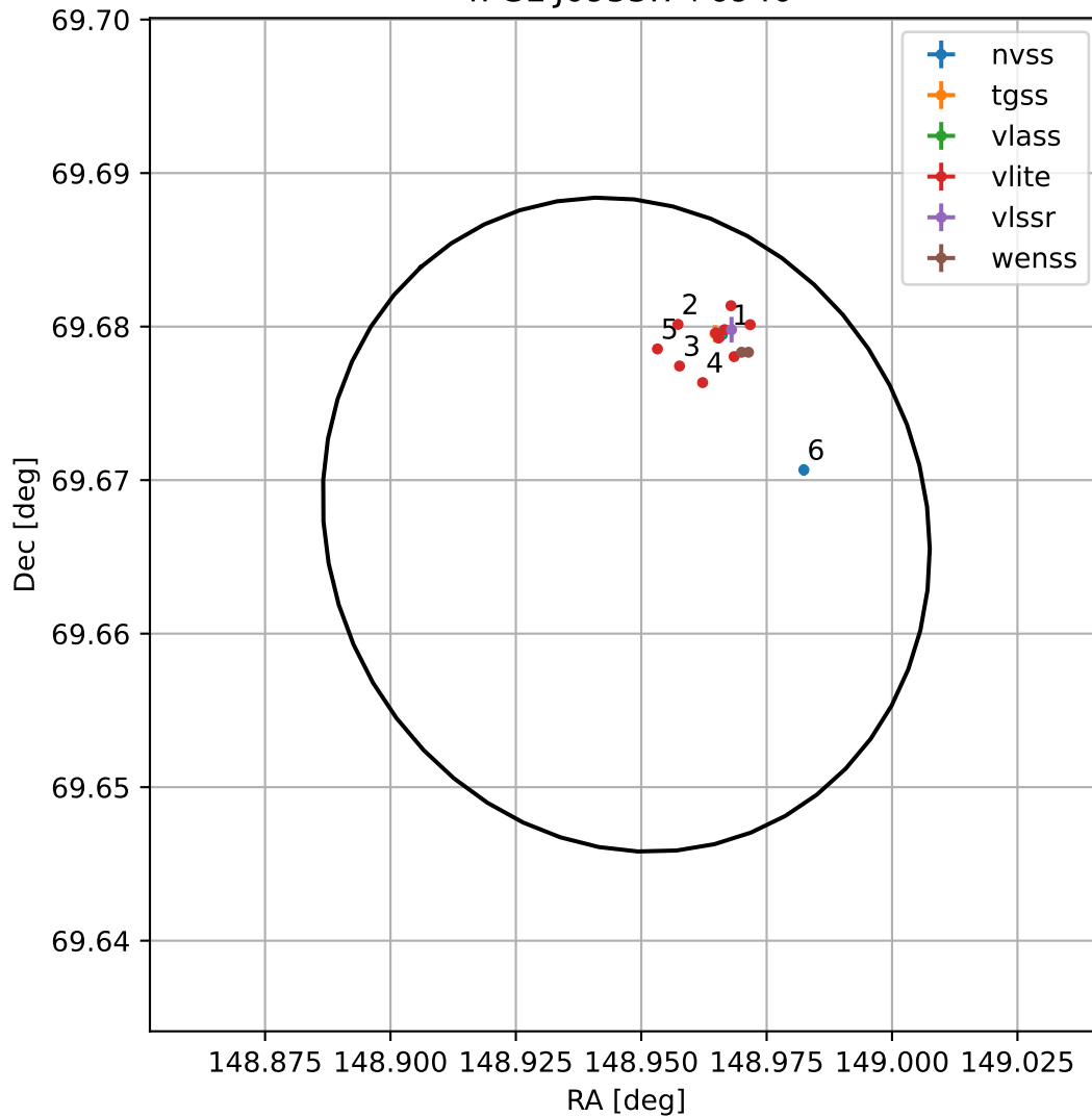
4FGL J0955.7+6940
