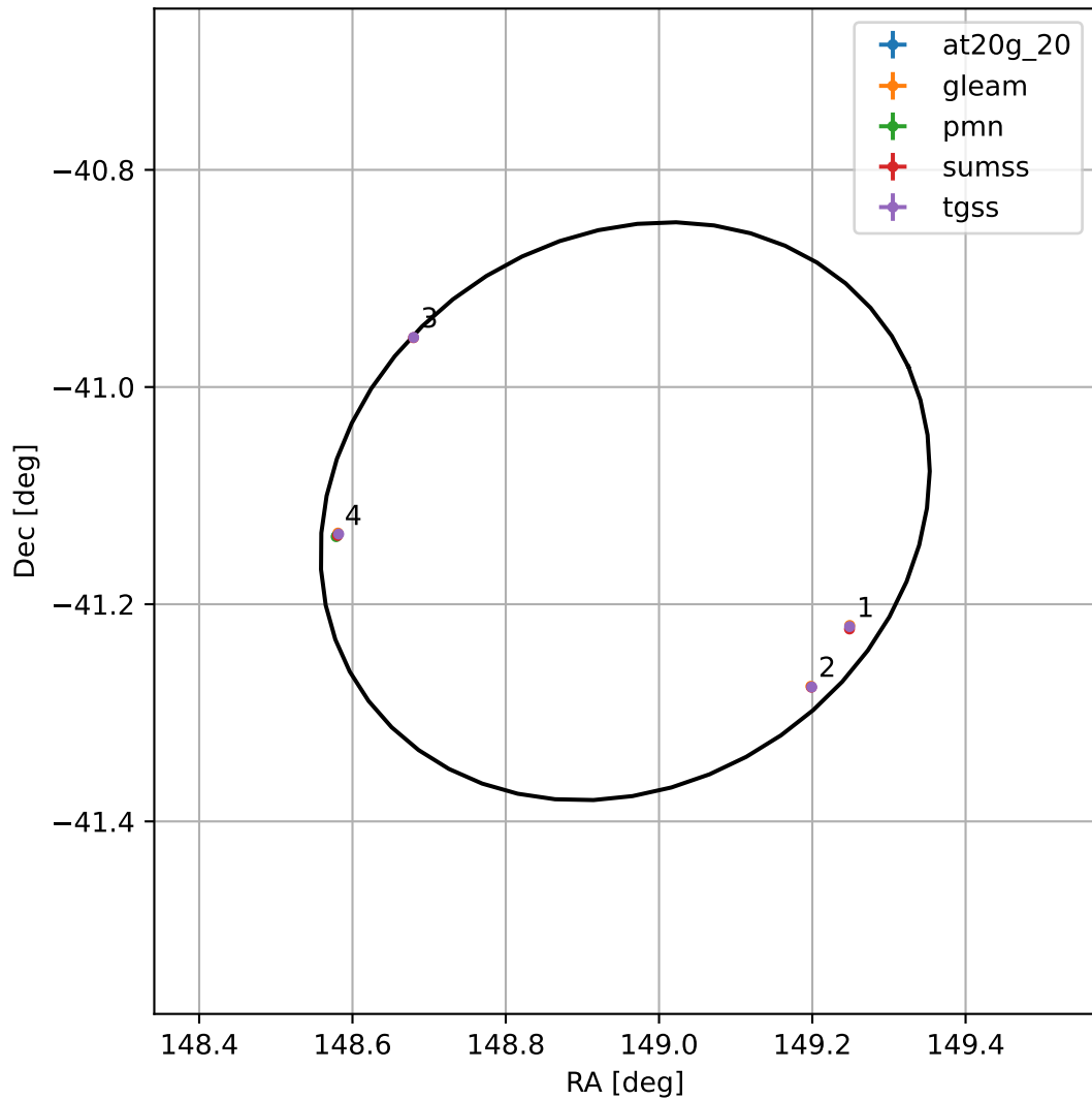
4FGL J0955.8-4106
