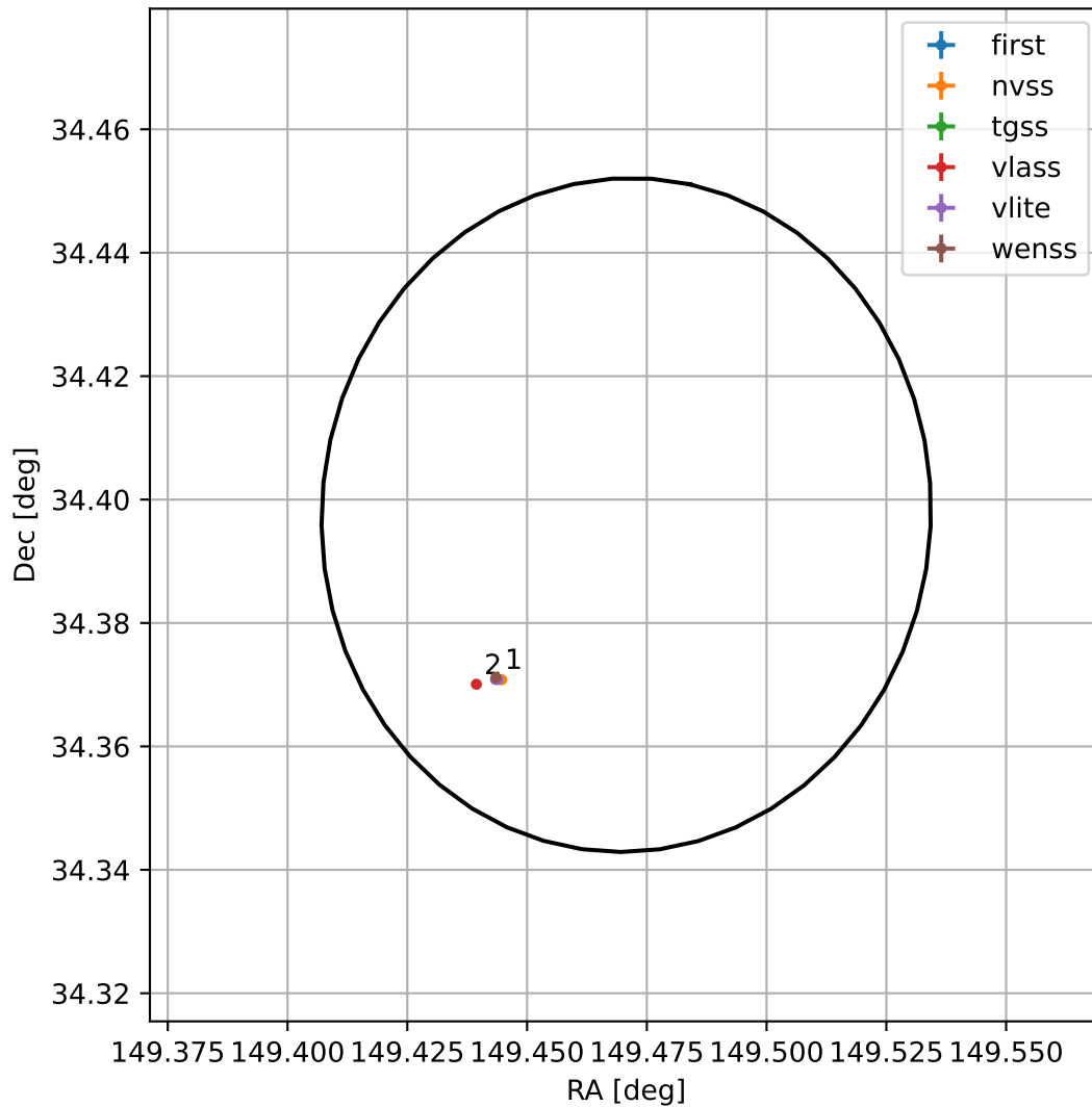
4FGL J0957.8+3423
