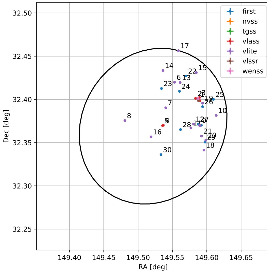
4FGL J0958.0+3222
