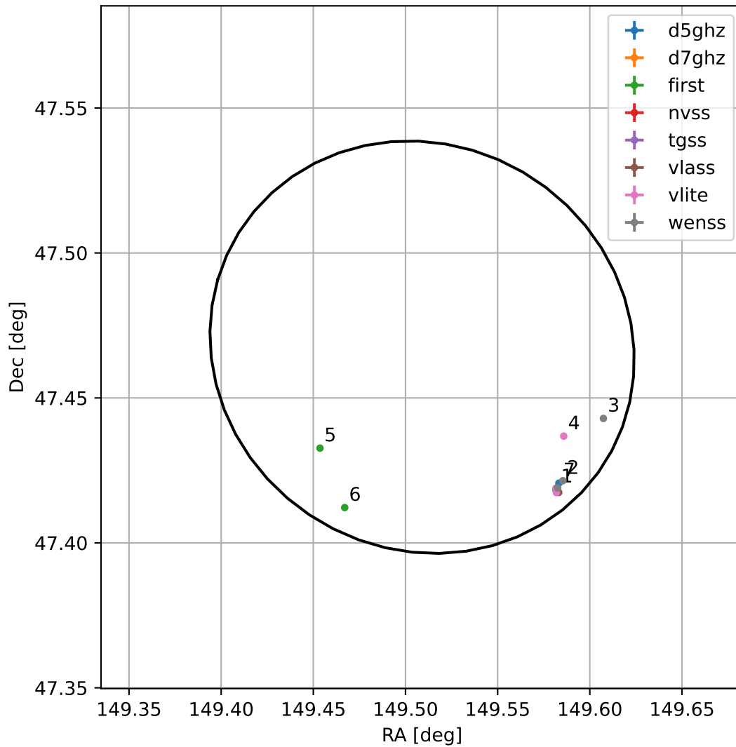
4FGL J0958.0+4728
