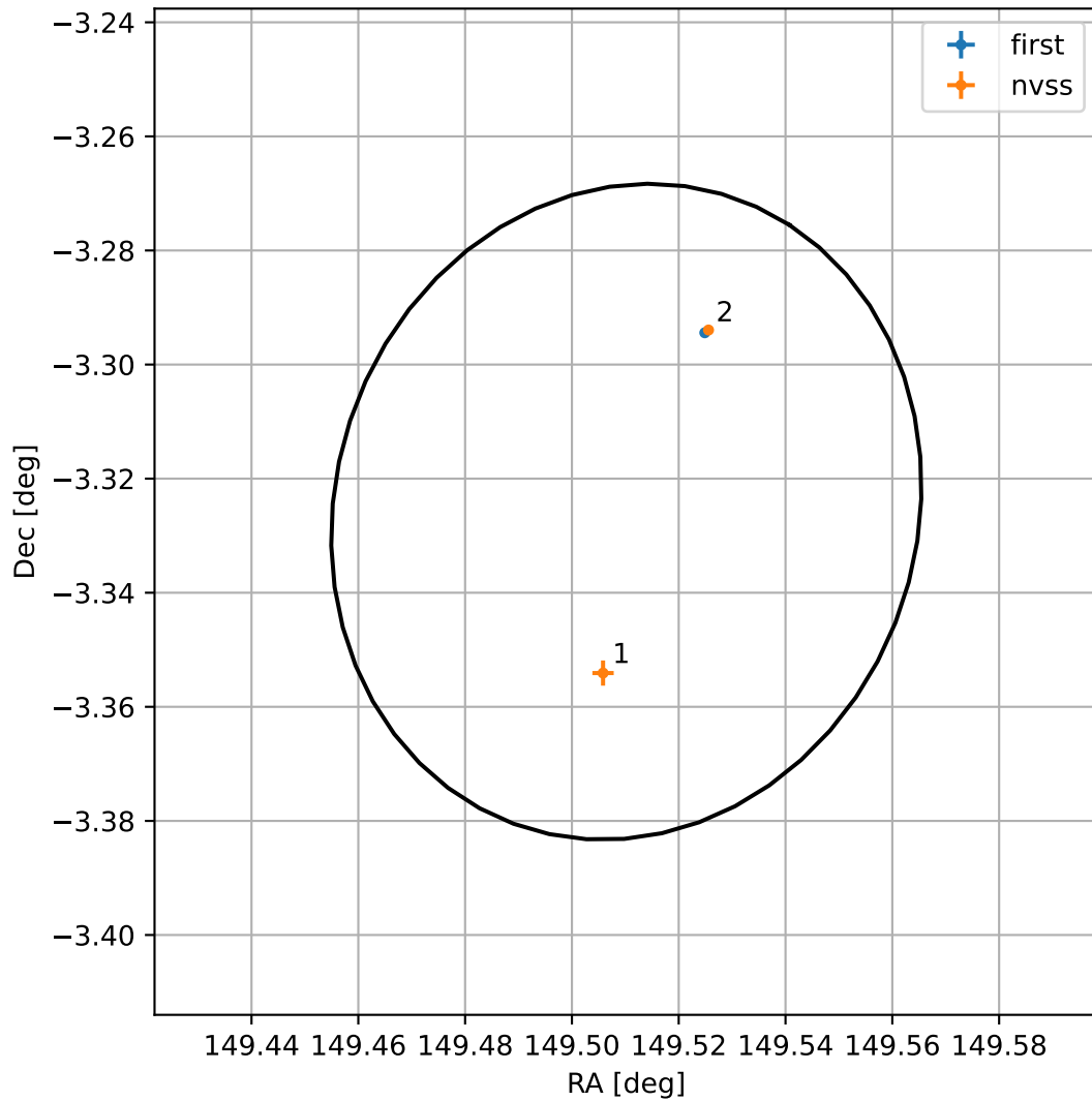
4FGL J0958.0-0319
