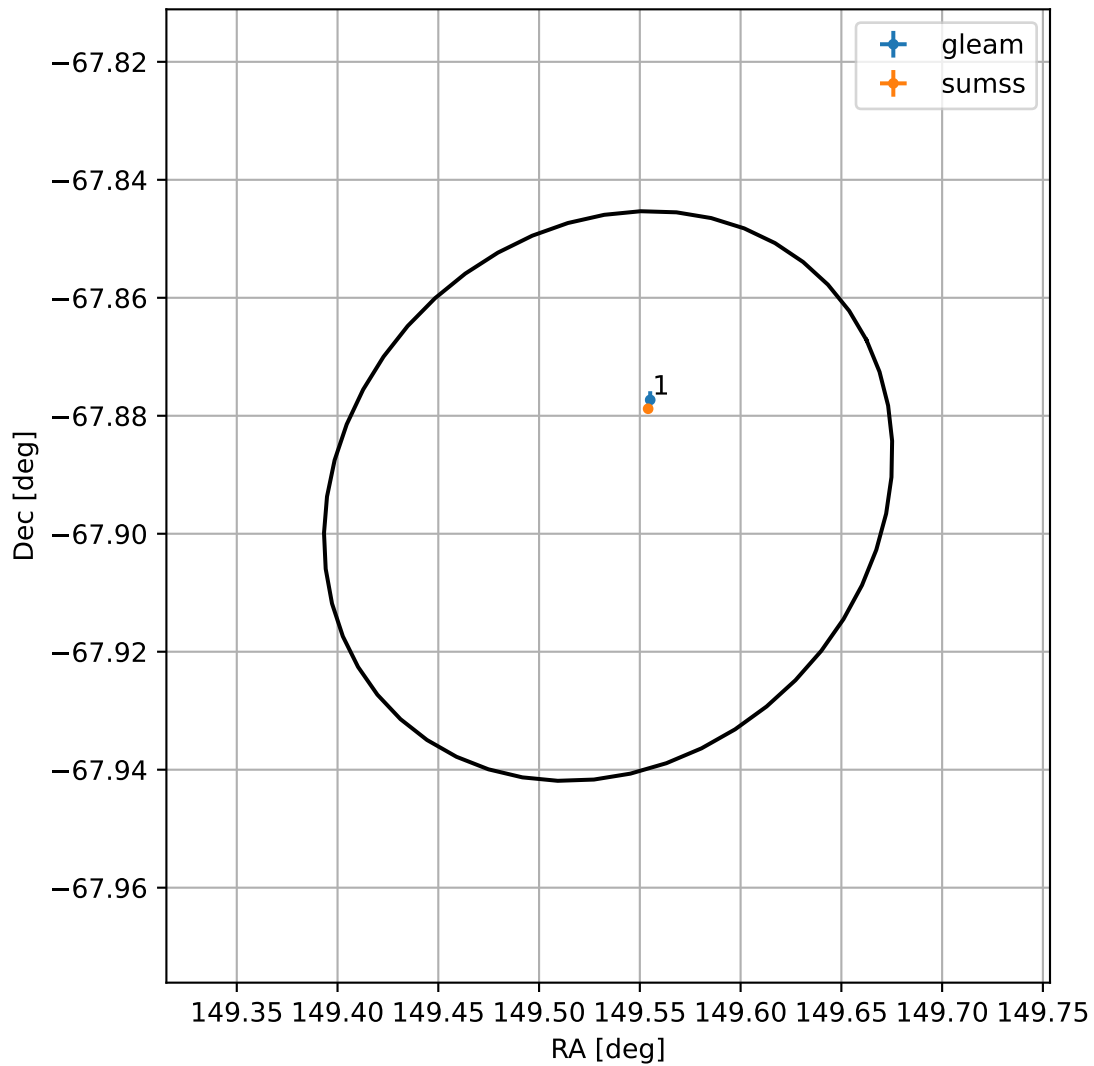
4FGL J0958.1-6753
