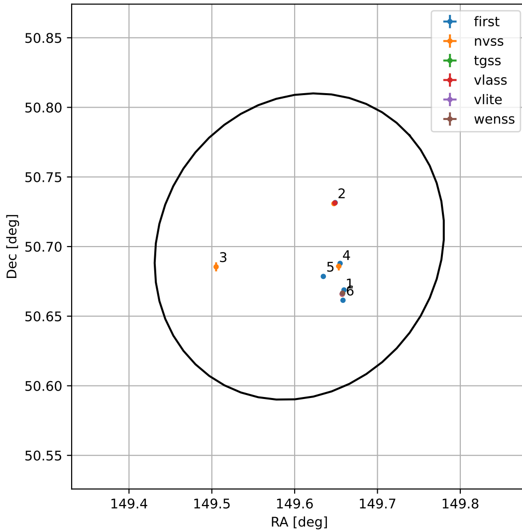
4FGL J0958.4+5042
