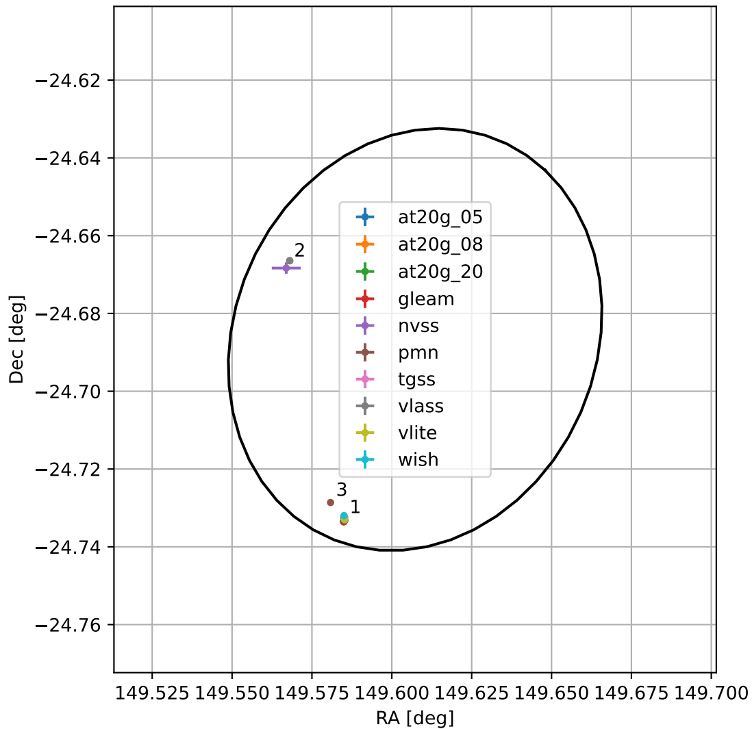
4FGL J0958.4-2441
