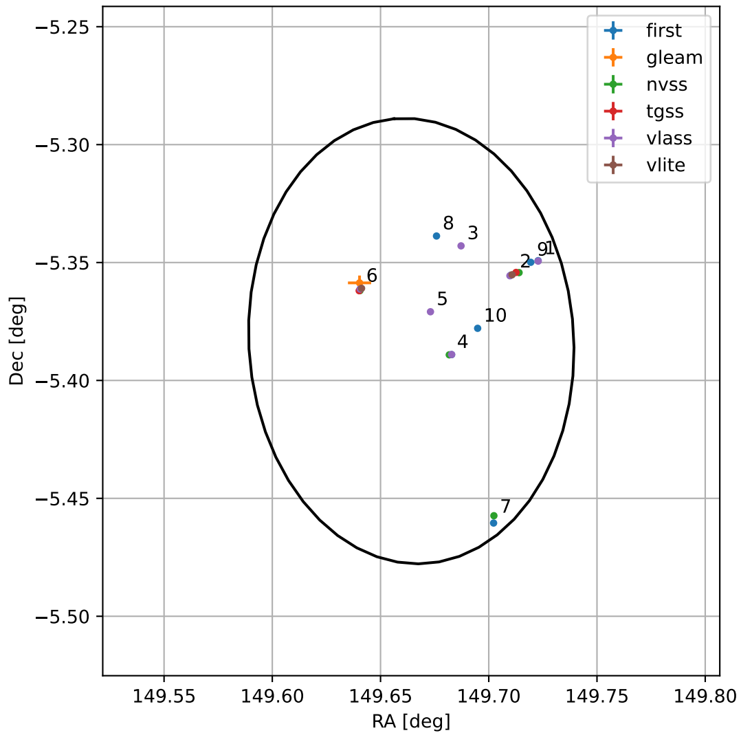
4FGL J0958.6-0522
