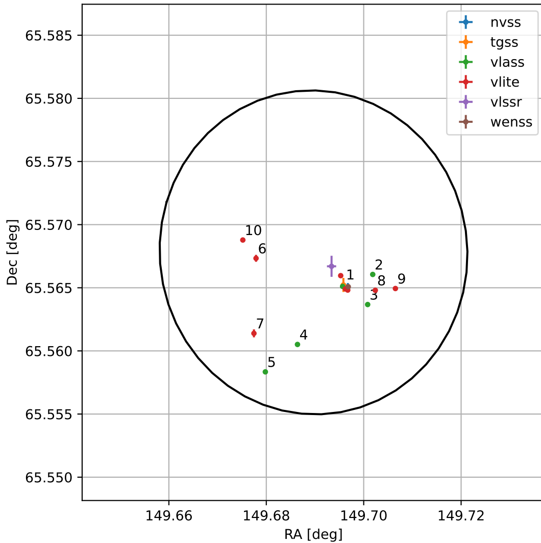
4FGL J0958.7+6534
