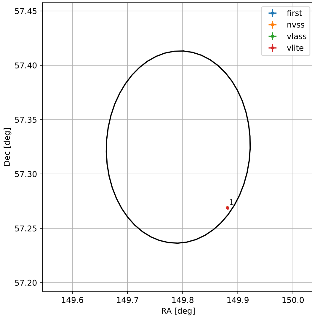
4FGL J0959.1+5719
