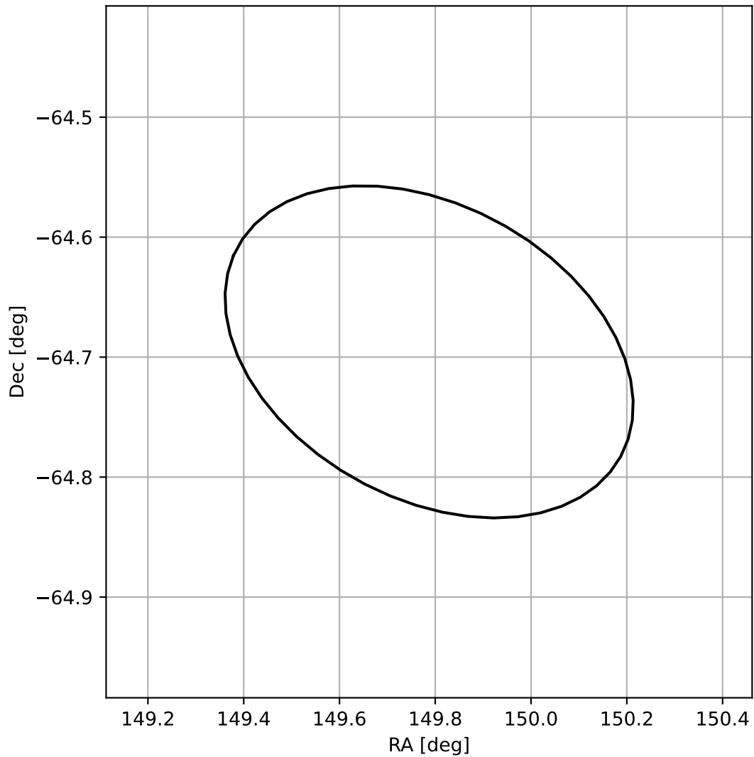
4FGL J0959.1-6441
