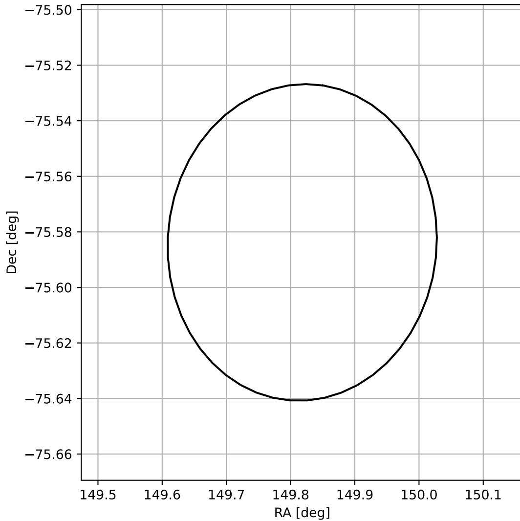
4FGL J0959.2-7535
