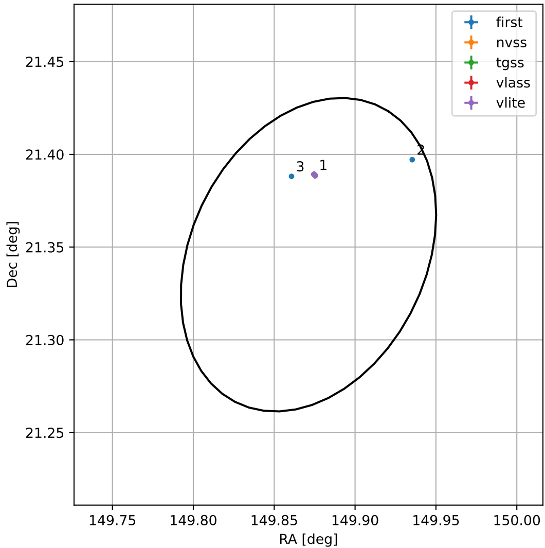
4FGL J0959.4+2120
