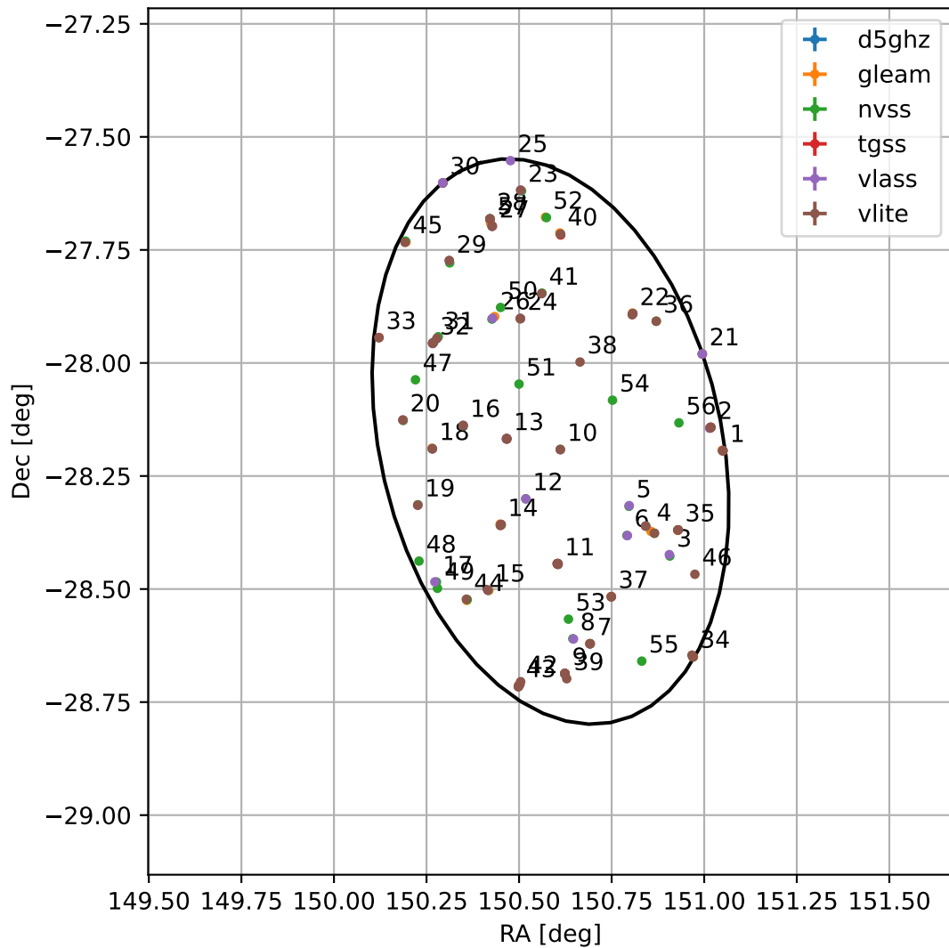
4FGL J1002.3-2810
