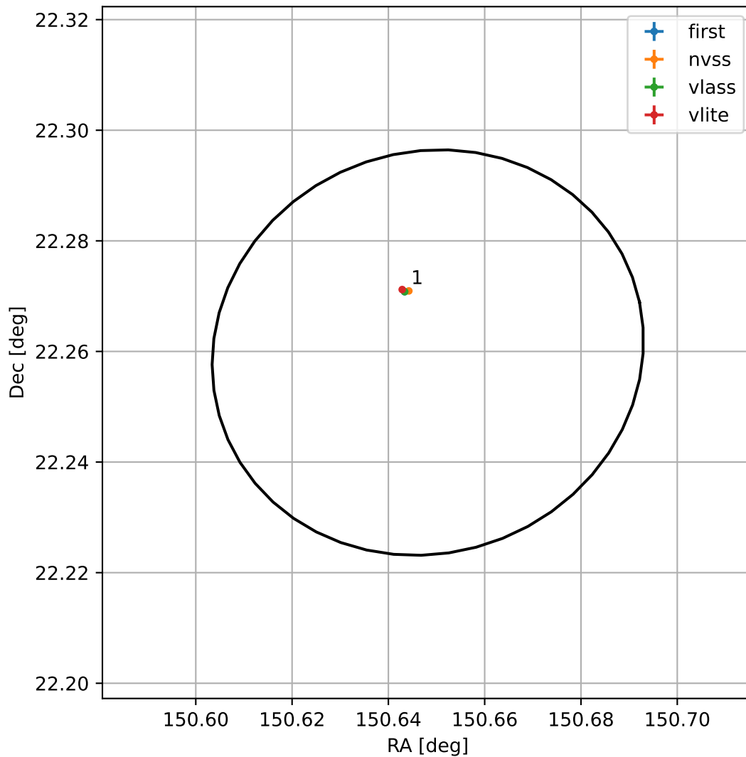
4FGL J1002.5+2215
