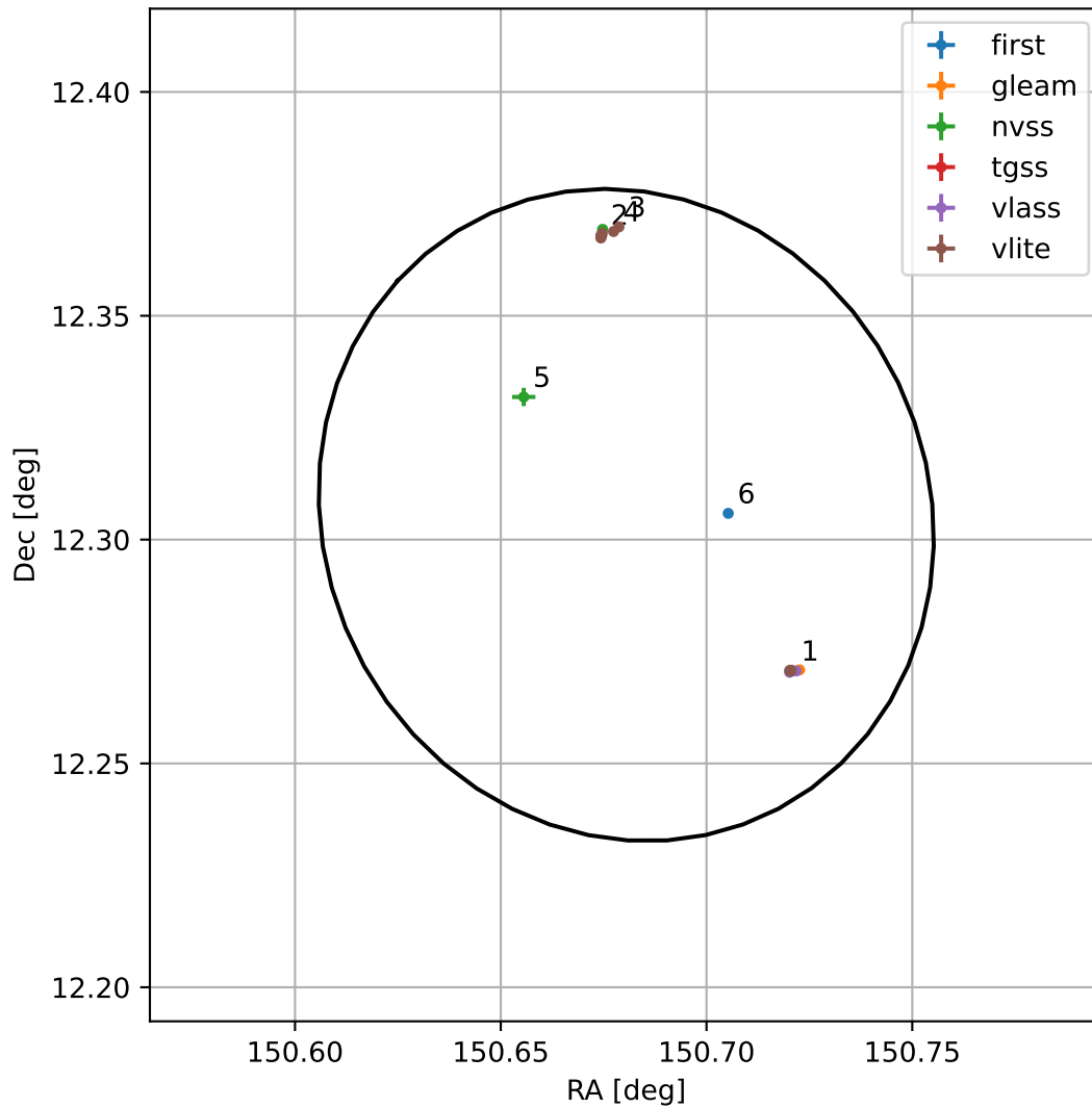
4FGL J1002.7+1218
