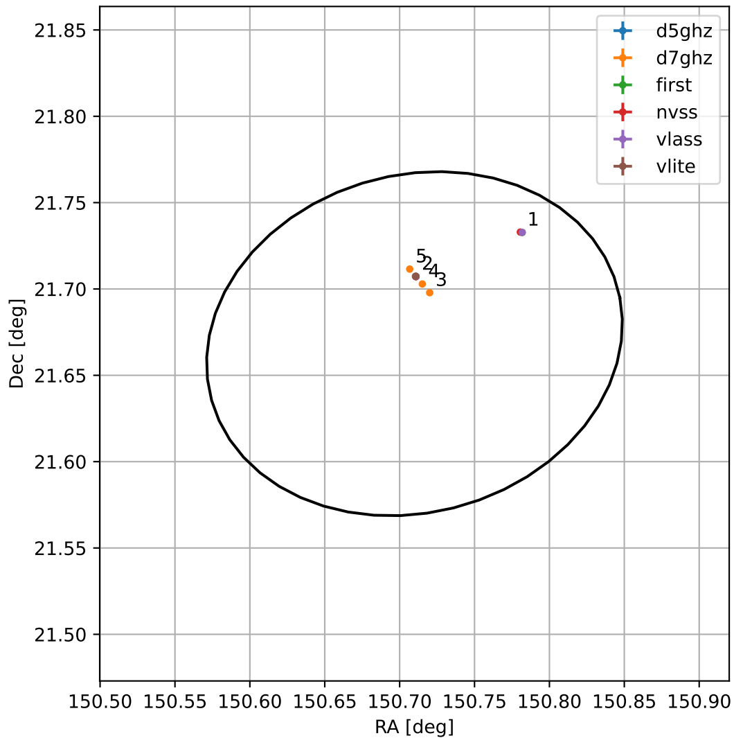
4FGL J1002.8+2140
