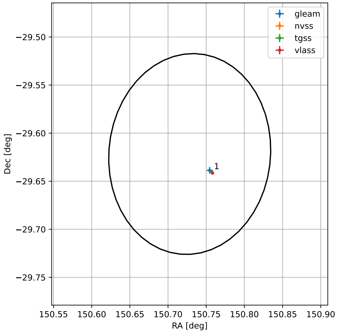
4FGL J1002.9-2937
