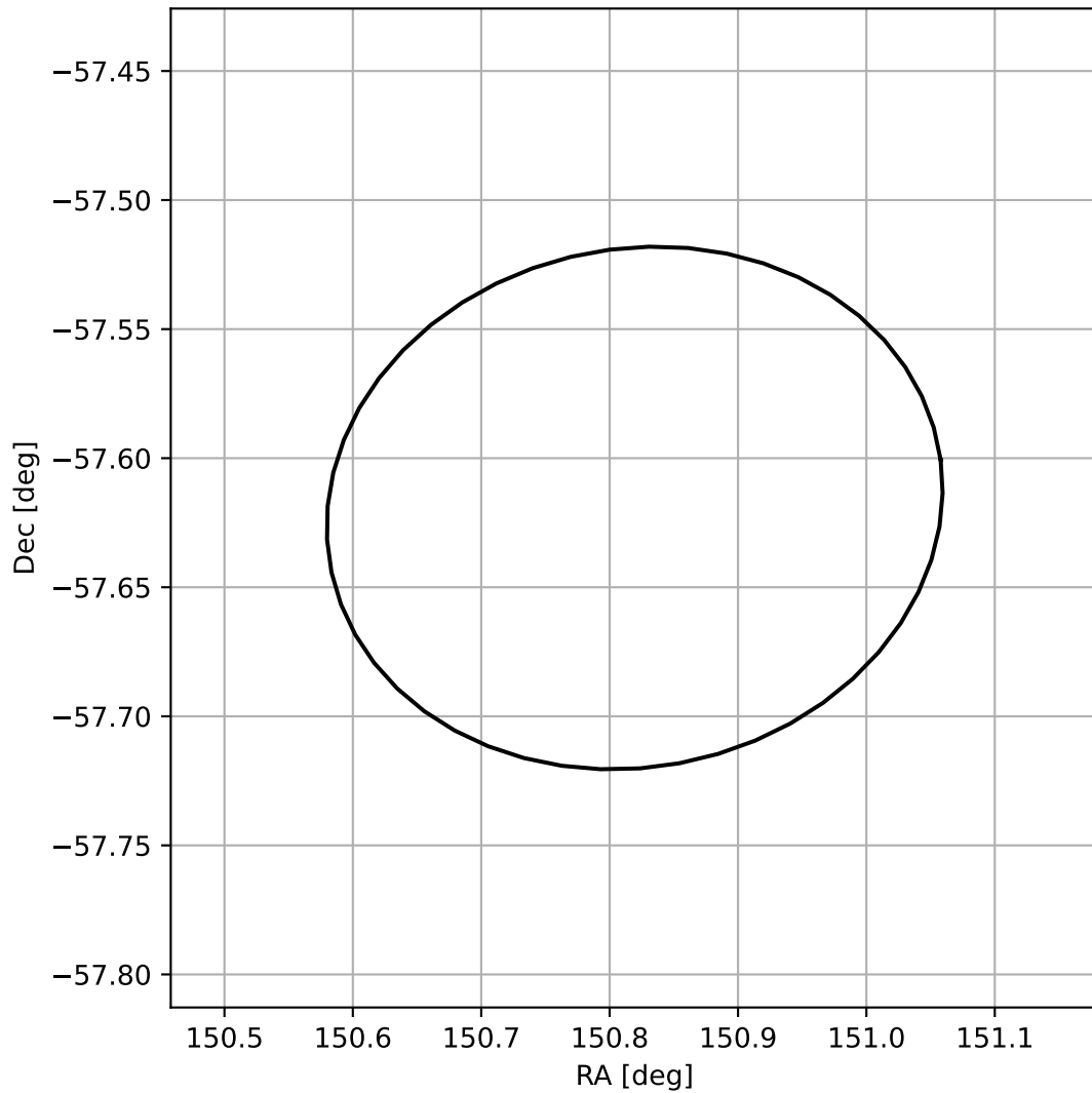
4FGL J1003.2-5737
