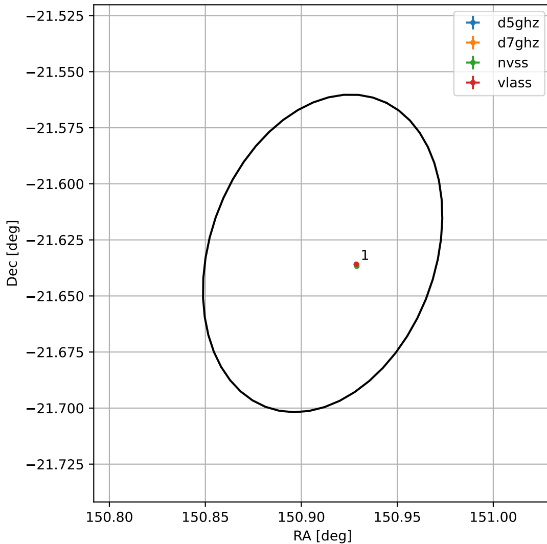
4FGL J1003.6-2137
