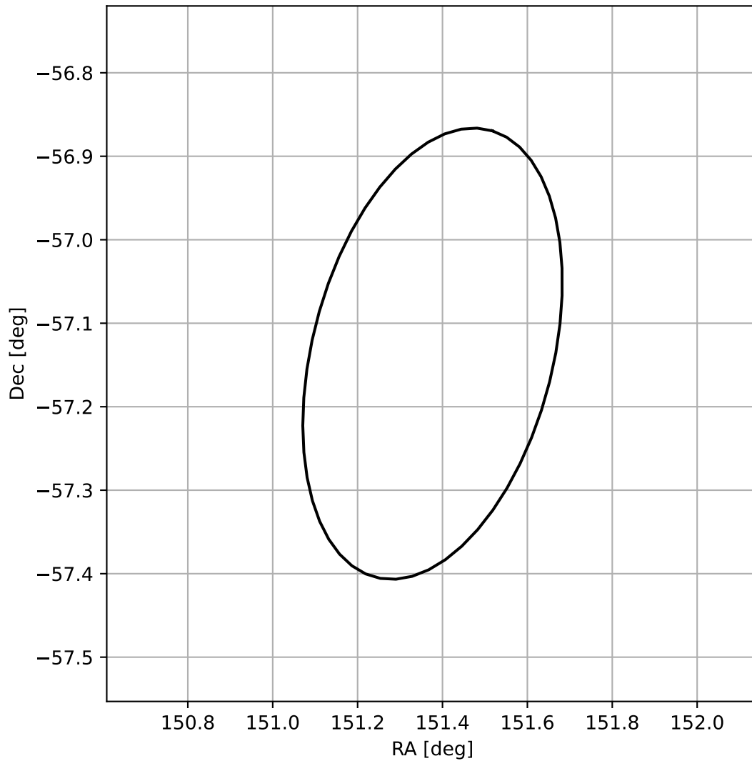
4FGL J1005.5-5708
