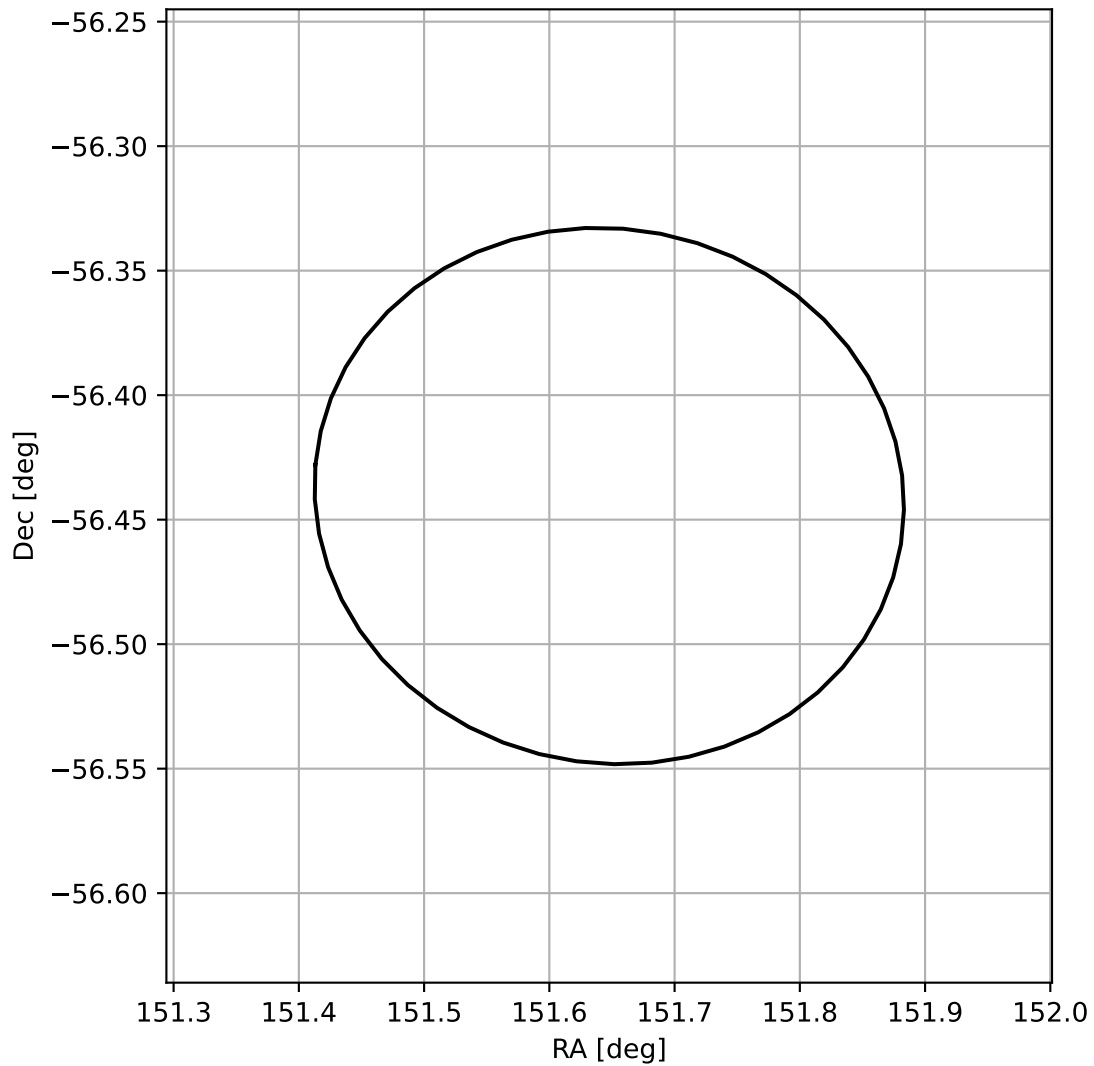
4FGL J1006.5-5626
