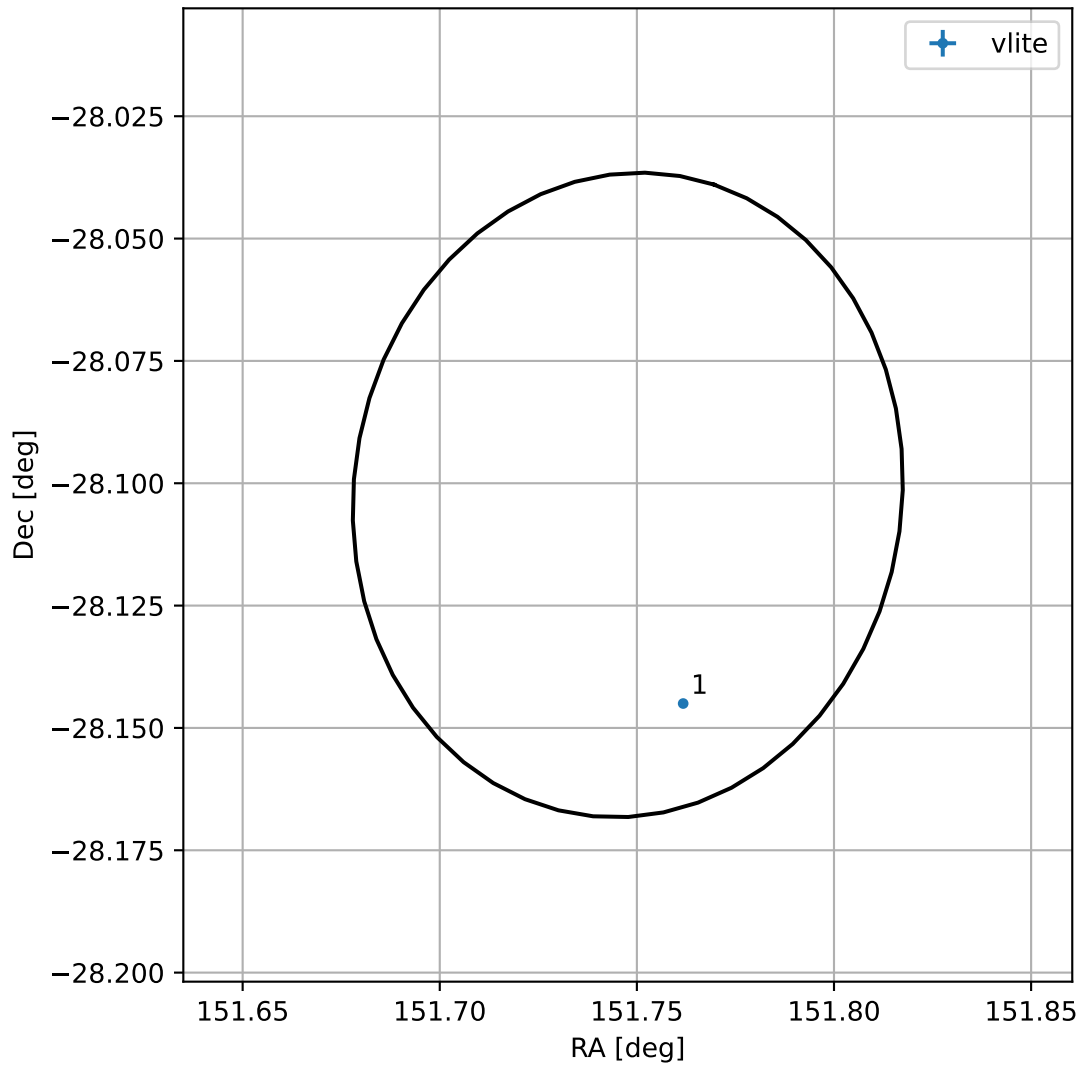
4FGL J1006.9-2806
