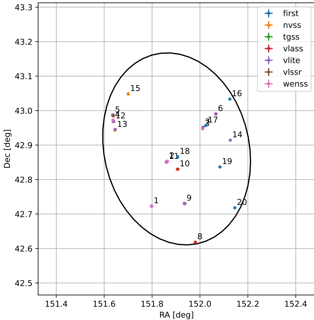
4FGL J1007.6+4253
