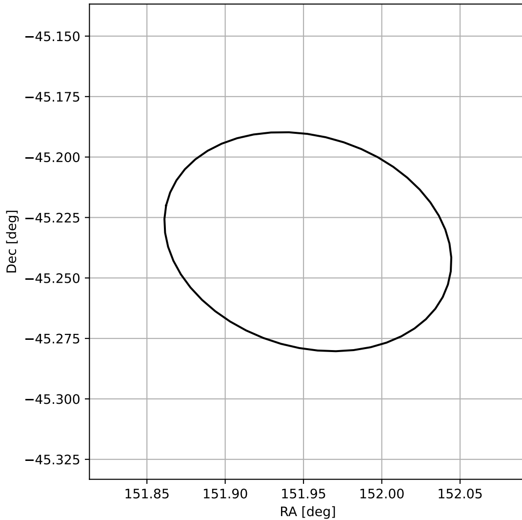
4FGL J1007.8-4514
