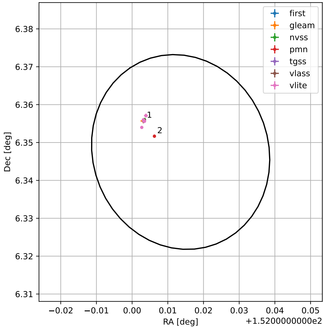
4FGL J1008.0+0620
