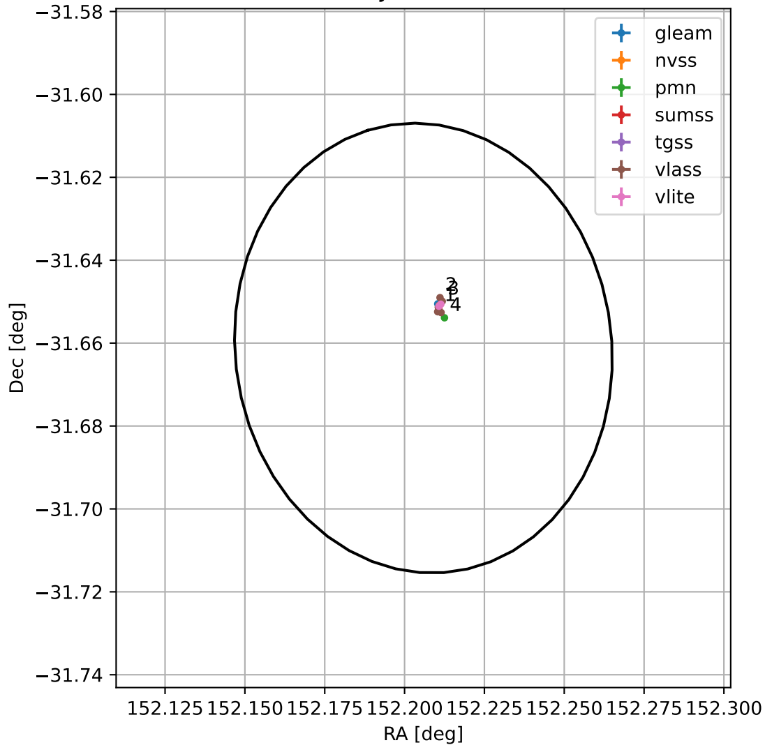
4FGL J1008.8-3139
