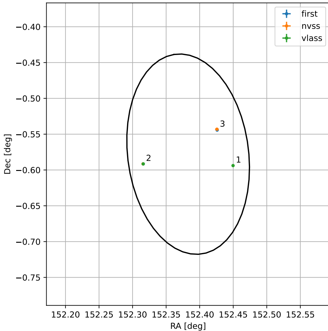
4FGL J1009.5-0034
