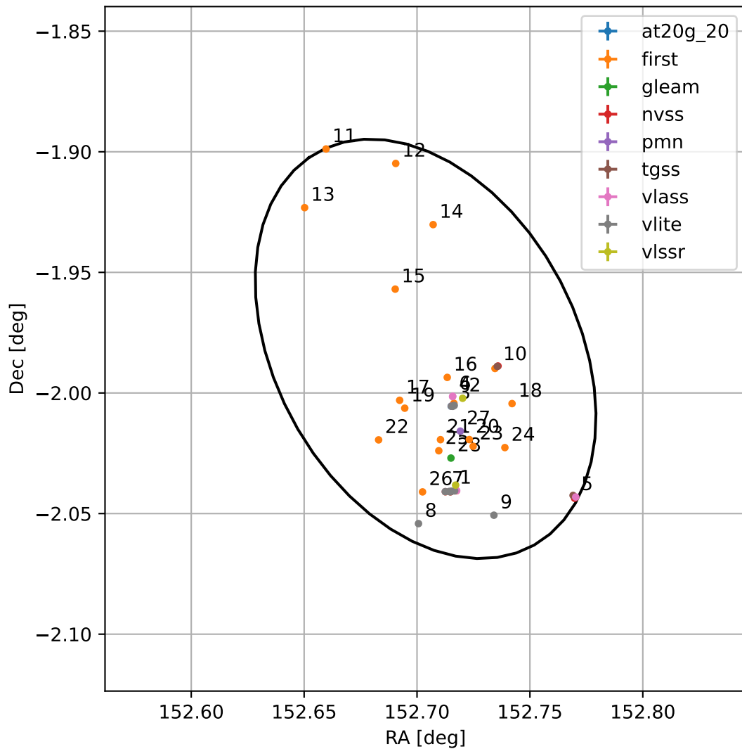
4FGL J1010.8-0158
